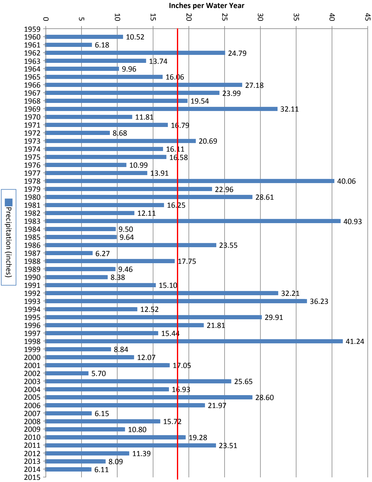
Figure B-1 Annual Precipitation at the SSFL, 1960 through 2014
